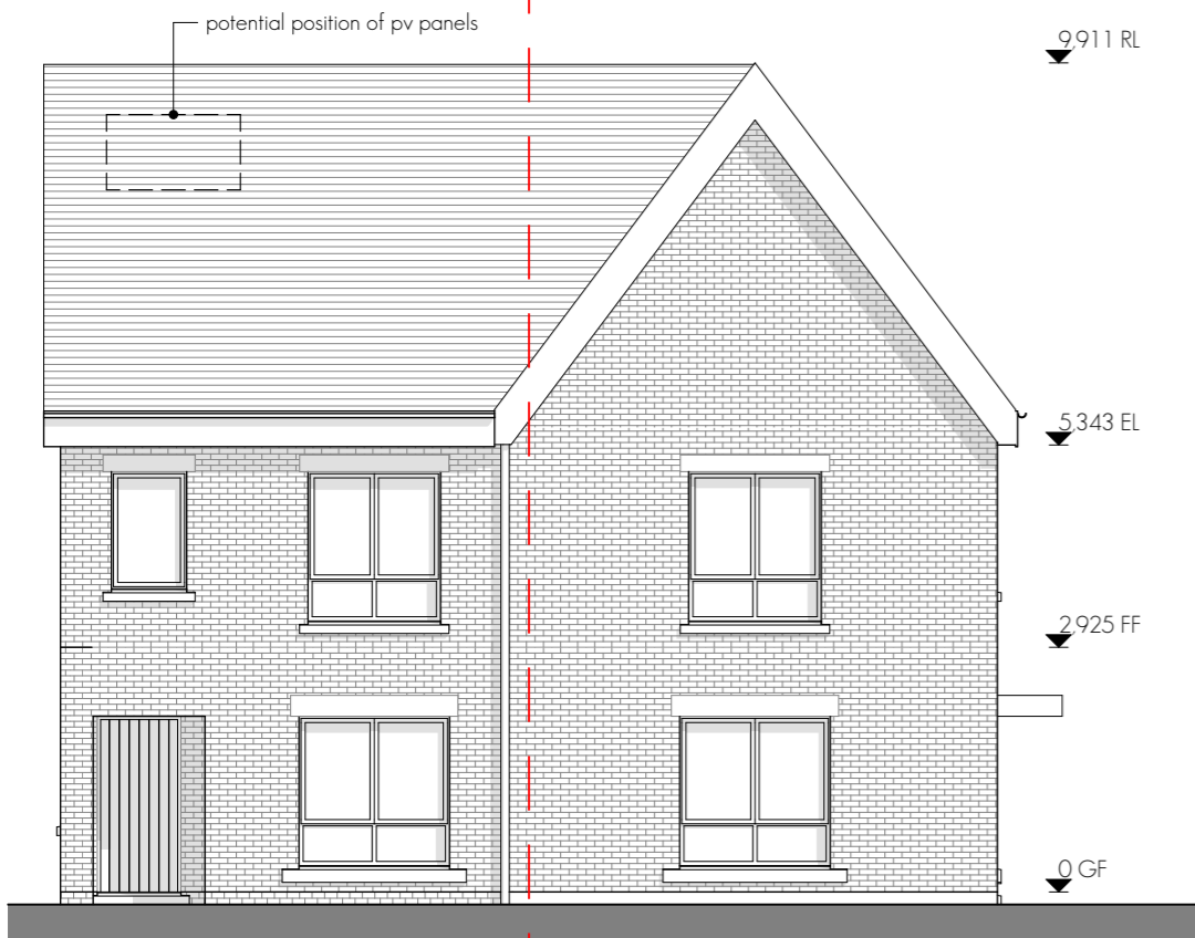
FRONT ELEVATION - B1/B3
